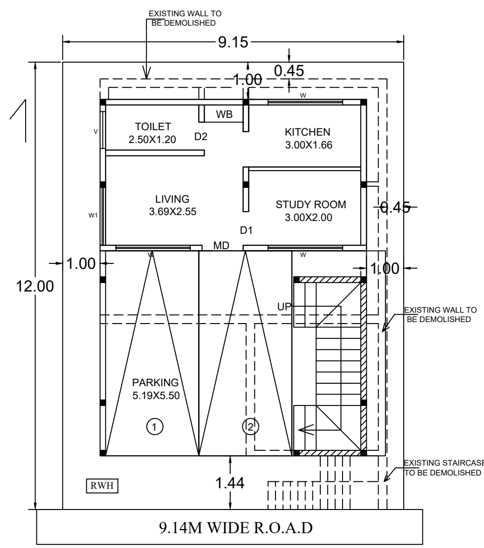
ALTERATION IN EXISTING GROUND FLOOR PLAN
